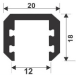
SGEP-01 For Glass Door, Size : 10 Ft. & 16 Ft.
