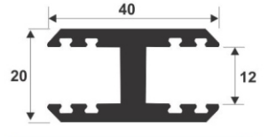
SGEP-04 For Glass Door Partion, Size : 10 Ft. & 16 Ft.
