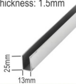
SUC-01 (CP) 'U' Channel (For Fixed Glass) Available in 10 Ft. Thickness: 1.5mm
