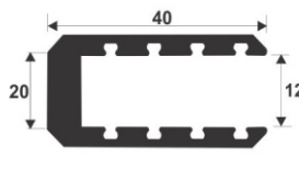
SGEP-03 For Glass Door, Size : 10 Ft. & 16 Ft.
