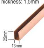
SUC-01 (Rose Gold) 'U' Channel (For Fixed Glass) Available in 10 Ft. Thickness: 1.5mm
