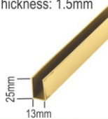
SUC-01 (Gold) 'U' Channel (For Fixed Glass) Available in 10 Ft. Thickness: 1.5mm
