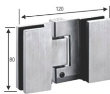
SCSF-3 Glass to Glass Hinge
